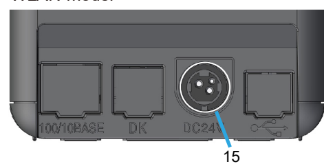
WLAN-model
