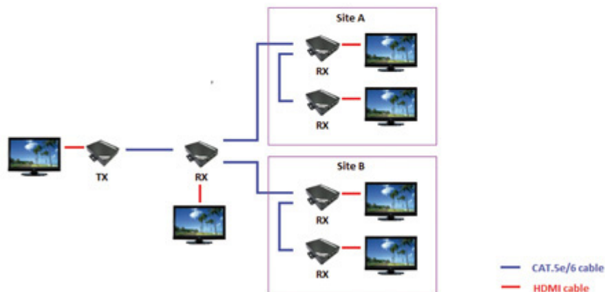
(3) Single Source with Multiple Receivers Cascaded
