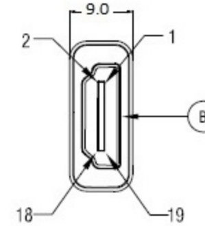
HDMI A Female
