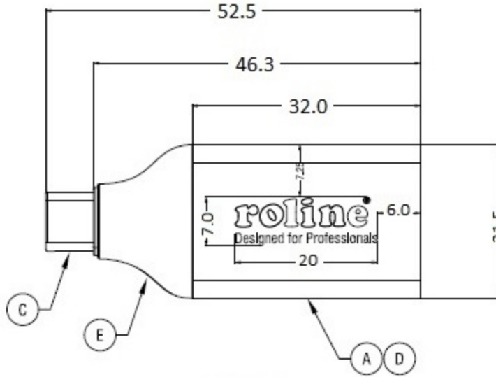
USB Type C Male
