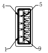
USB 3.0 A Male
