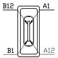
USB Type C Female
